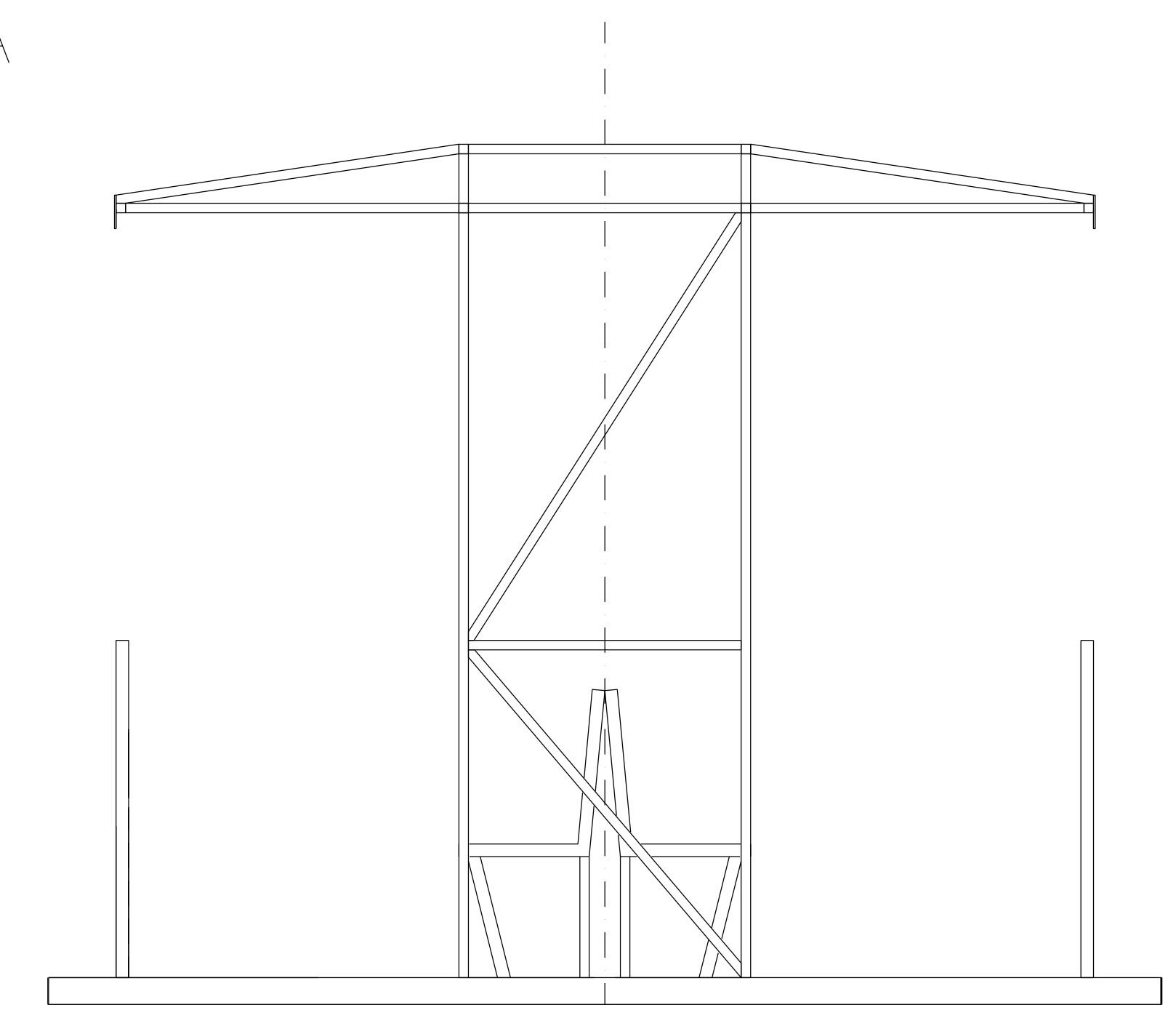
PART SECT B-B LOOKING AFT
