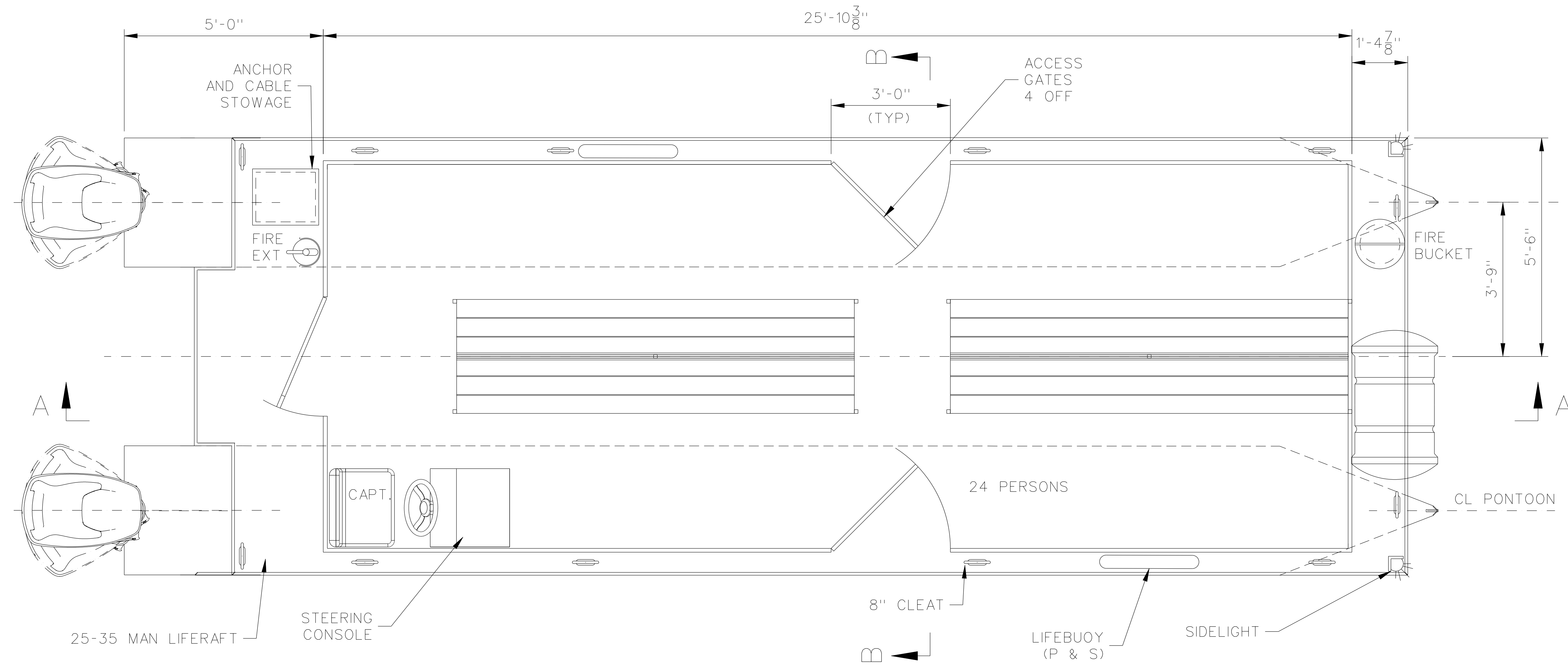
PLAN AT MAIN DECK
