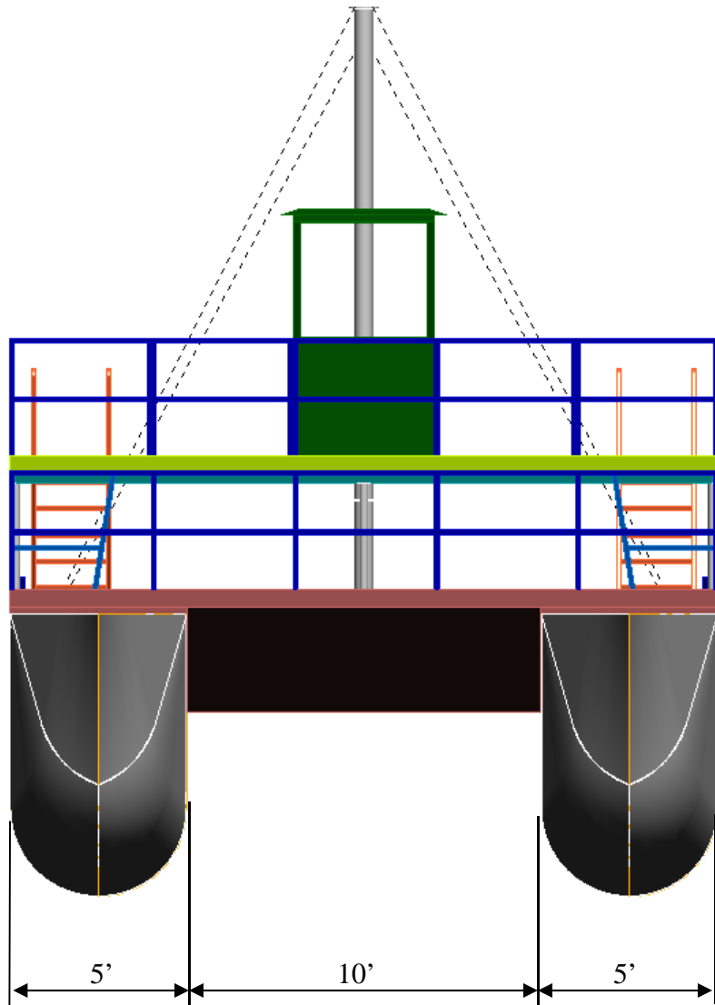
FRONT VIEW
