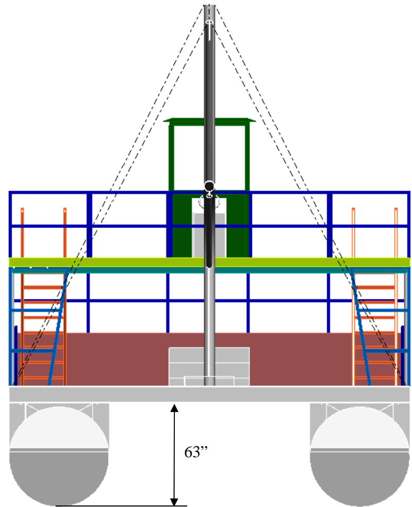
REAR VIEW
